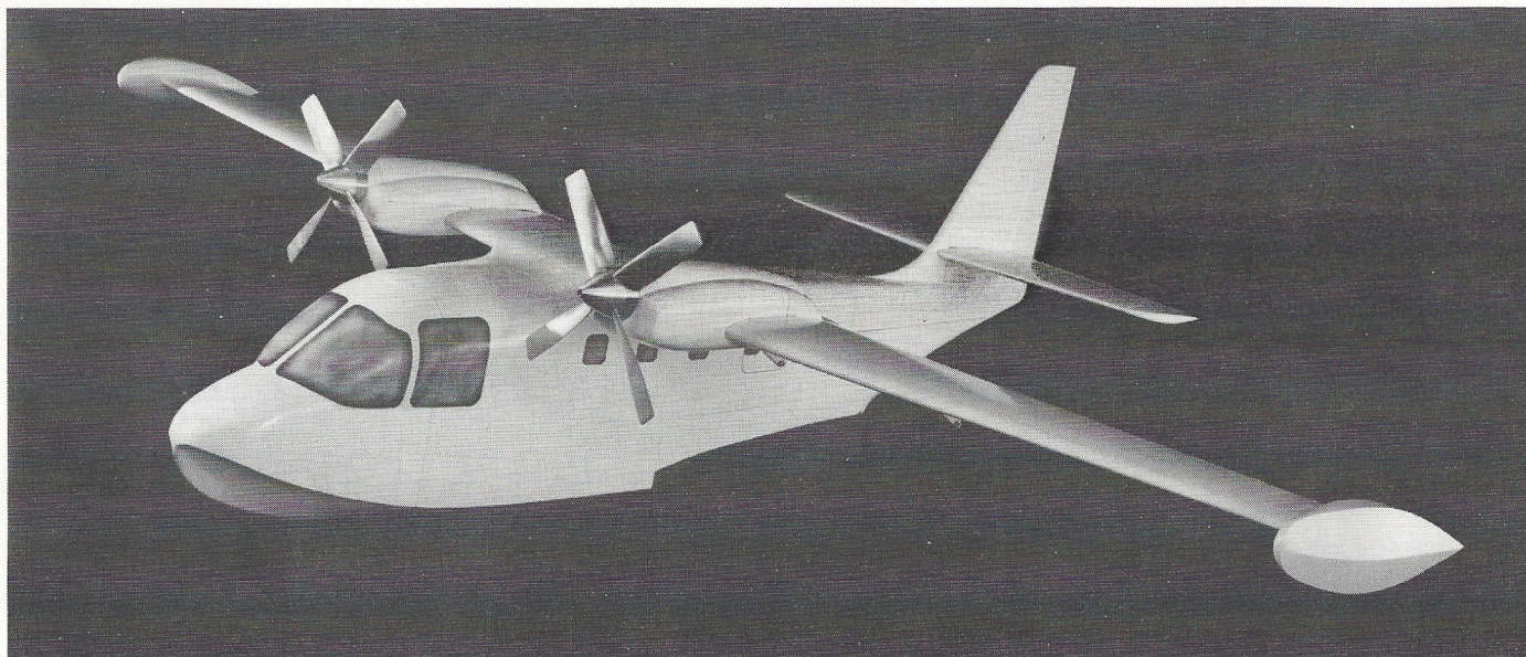
Grumman Aerospace Design 711 started wind tunnel testing recently with a 1/4-scale model to examine the lift, drag and moment characteristics of the baseline configuration. The 10-place amphibian is designed to incorporate either piston or turboprop engines.
